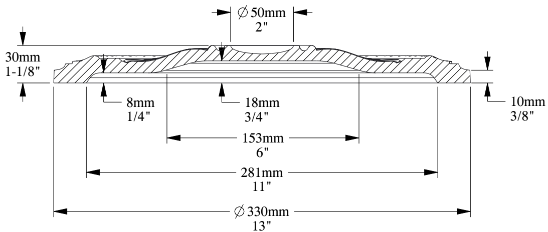
SECTION A-A SCALE 33:100
